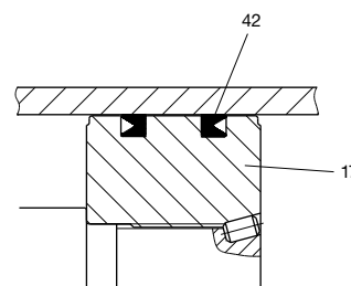
Lipseal Piston
