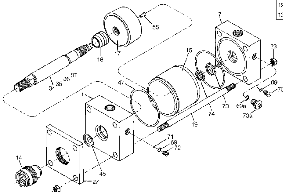
Lipseal Piston
